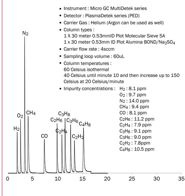
CHROMATOGRAM #6
